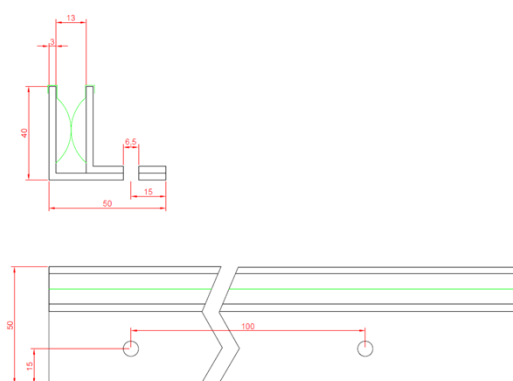
Hybrid EPP absorber base Fix unit Work with M4x50 screw
